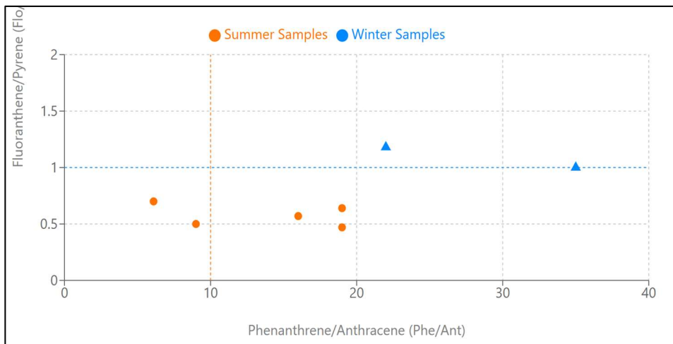
Fig. 5: Diagnostics ratios for PAH source apportionment in the Shatt al-Arab River.
