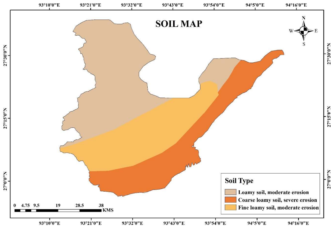
Fig. 8: Soil map.
