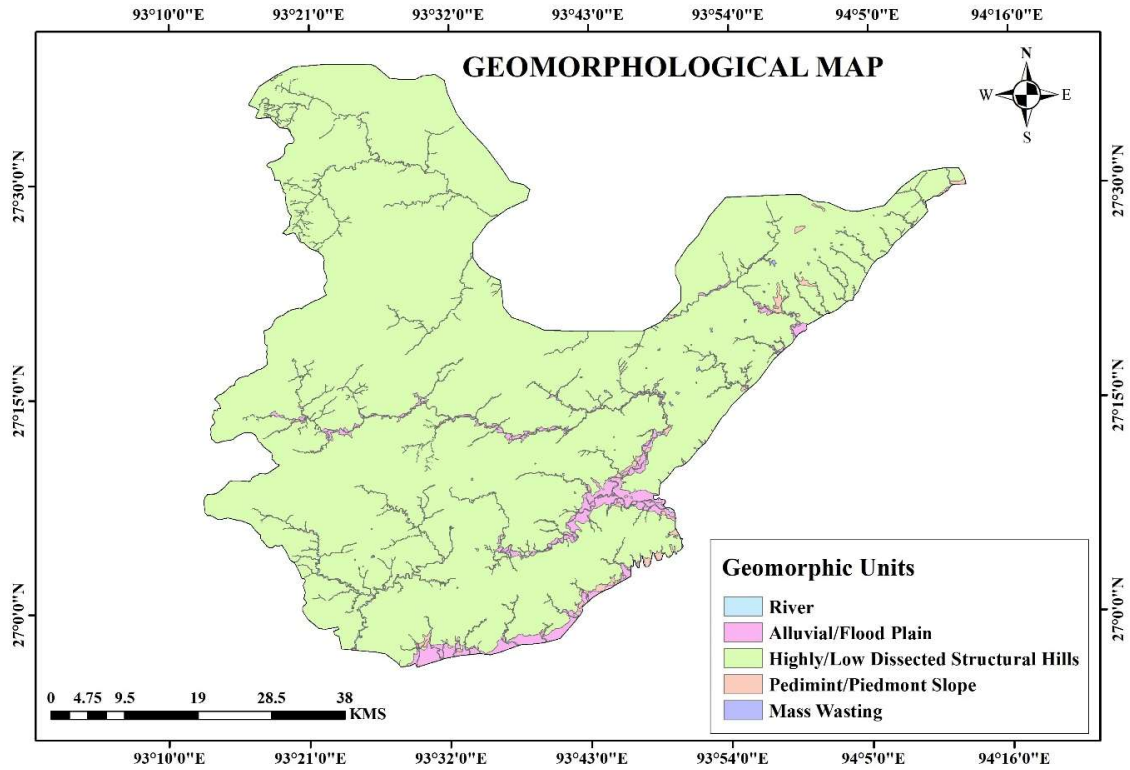
Fig. 7: Geomorphology.
