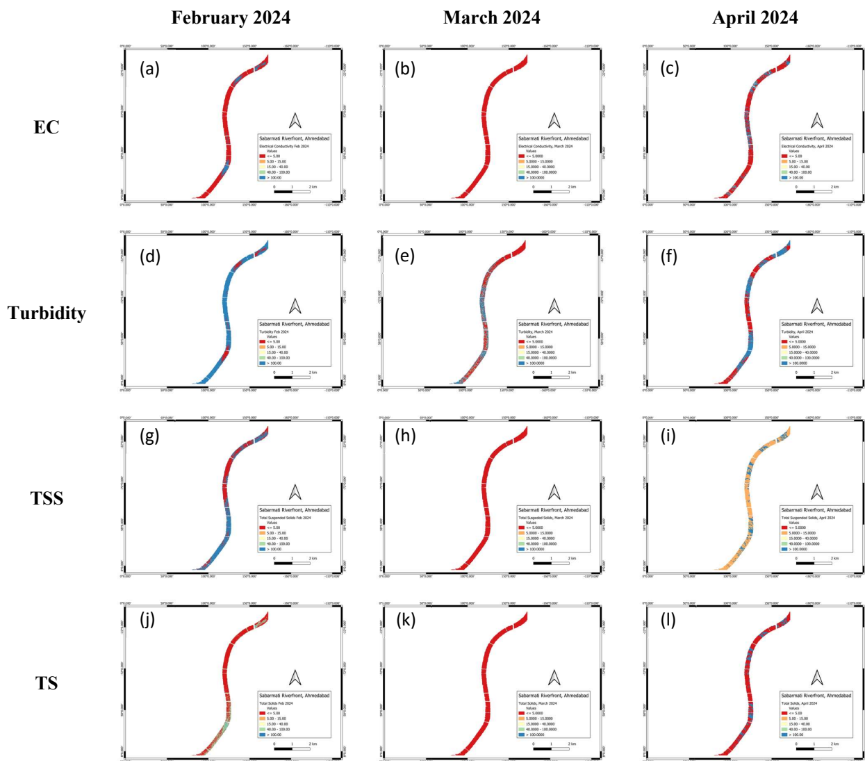
Fig. 4: Represents the spatial distribution of optically active water characteristics.
