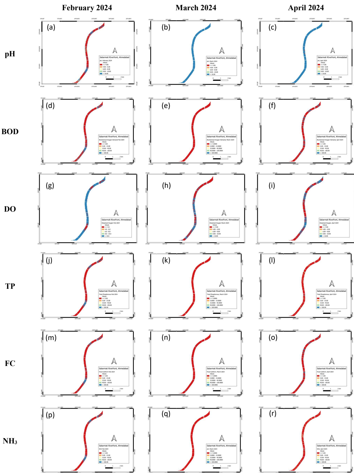
Fig. 5: Represents the spatial distribution of non-optically active water characteristics.
