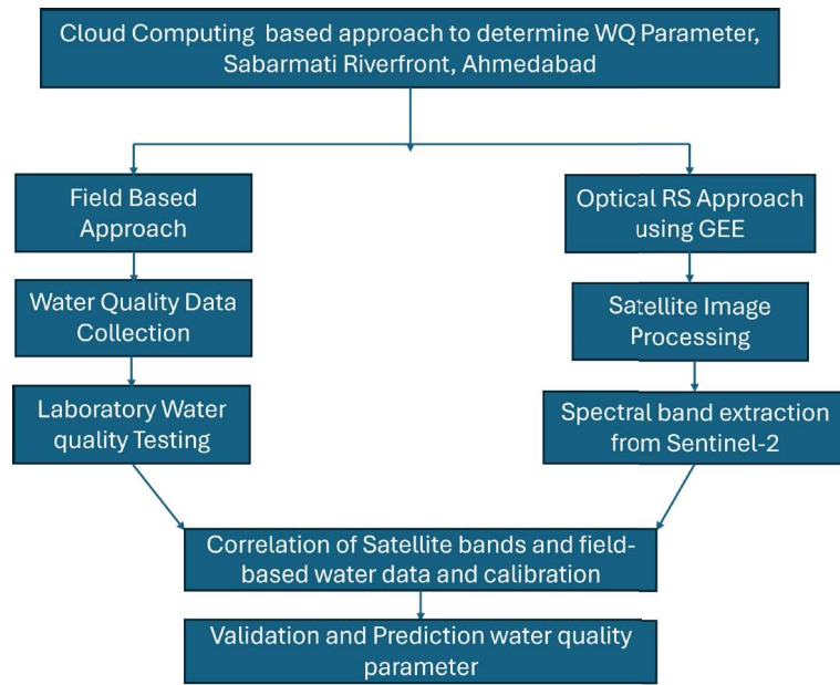
Fig. 3: A broad framework of methodology.
