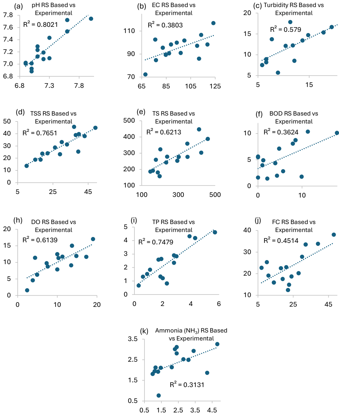
Fig. 6: R^2 values for the accuracy assessment of remote-sensing derived v/s experimental water quality concentrations.
