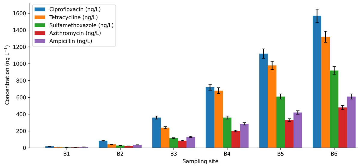
Fig. 2: Clustered bar chart showing measured antibiotic concentrations (ng L -1 ) across Bindal River sampling sites B1–B6.
