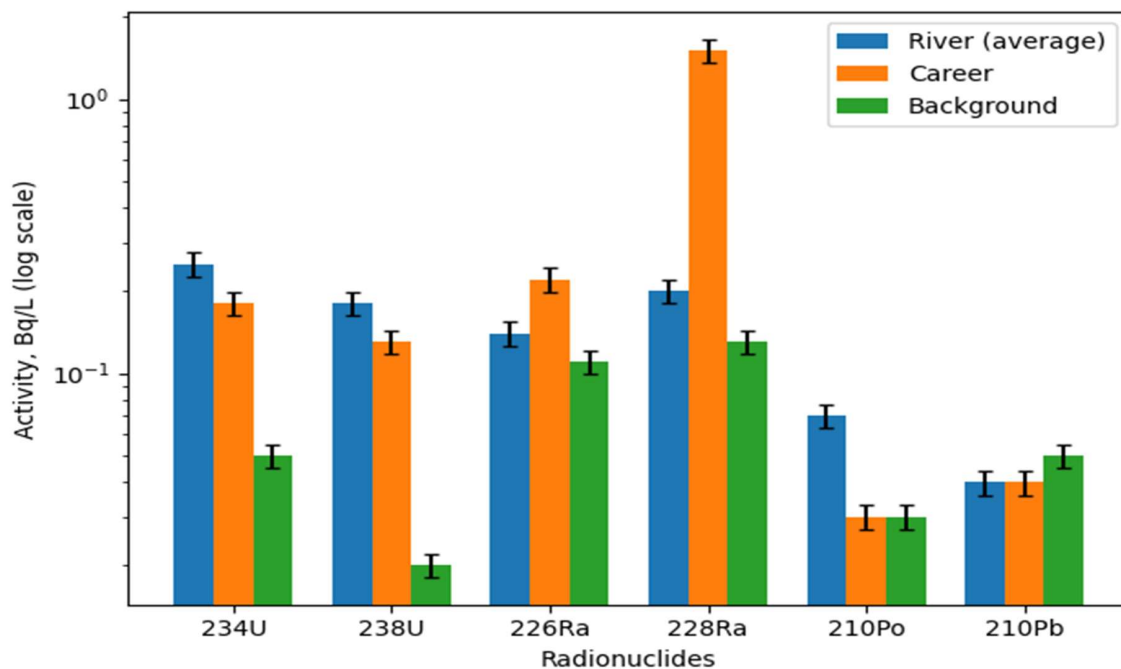
Fig. 3: Logarithmic distribution of radionuclide concentrations.
