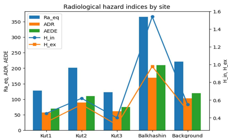
Fig. 4: Radiological hazard indices by sampling site.
