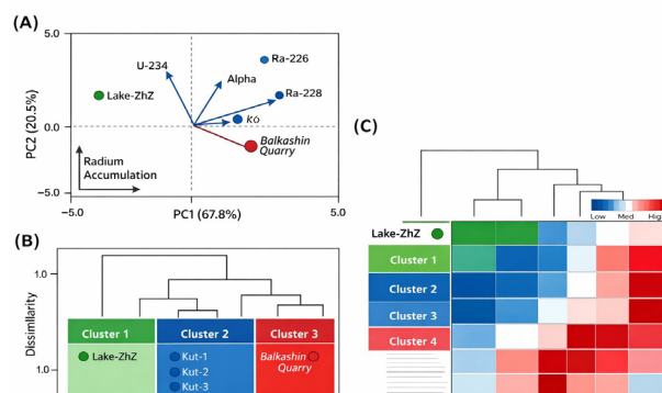
Fig. 5: Multivariate statistical analysis of the distribution of natural radionuclides at the investigated sampling sites: (A) principal component analysis (PCA), (B) hierarchical cluster analysis, (C) heatmap.
