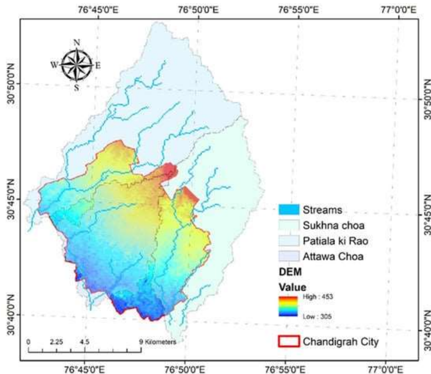
Fig. 2: Runoff diagram of Chandigarh.
