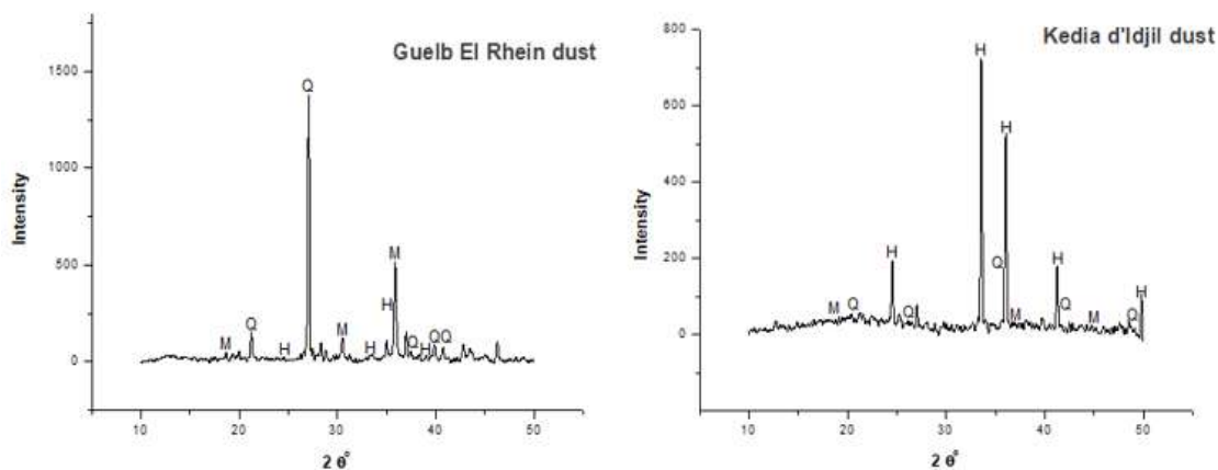
Fig. 4: X-ray diffraction diagrams for dust samples from Guelb El Rhein and Kedia d'Idjil. H, hematite; M, magnetite; Q, quartz.
