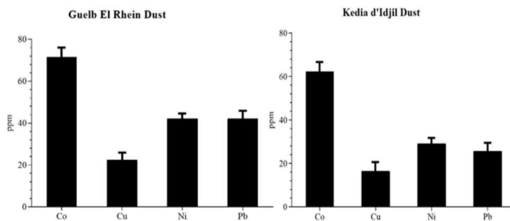
Fig. 5: Heavy metal (Co, Cu, Ni, and Pb) contents measured in the two iron ore dust types, Guelb El Rhein dust and Kedia d'Idjil dust.
