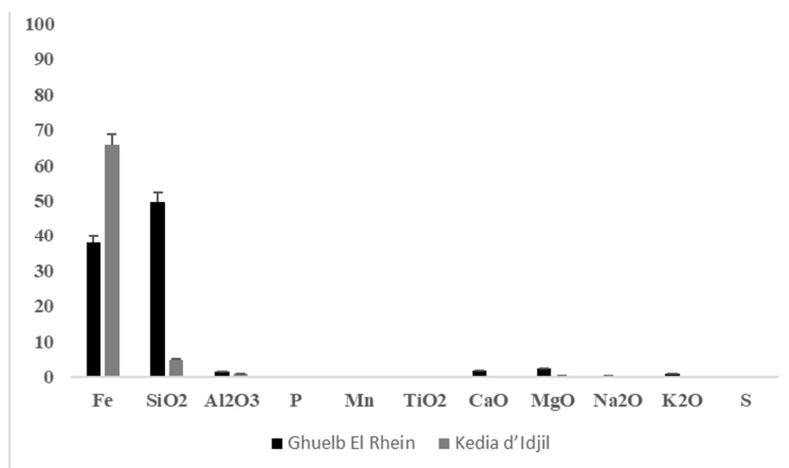
Fig. 3: Mean \pm standard deviation of percentage composition determined by X-ray fluorescence (XRF) analysis.
