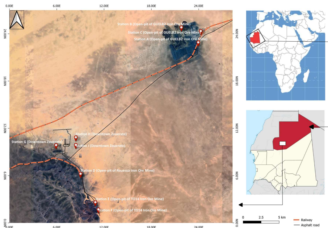
Fig. 1: Location of sampling stations within the National Industrial and Mining Company (SNIM) in the Tiris Zemmour region, Mauritania. Stations A, B, and C are located in the Guelb El Rhein mine along the Guelb 2 production circuit. Station D (Rouessa) and stations E and F (TO14 area) are situated in the Kédia d'Idjil mine. Stations G, H, and I are located in downtown Zouerate.
