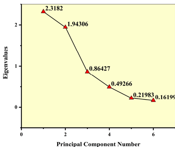
Fig. 7: Scree plot illustrating variance explained by principal components of total metals.
