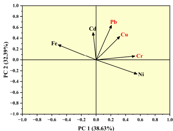
Fig. 6: Principal component analysis (PCA) loading plot of total heavy metals in Cauvery Delta wetland sediments.
