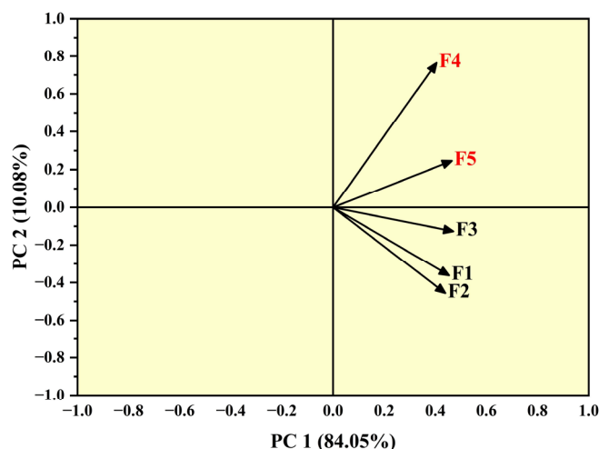
Fig. 4: Principal component analysis (PCA) loading plot of heavy metal speciation fractions (F1–F5) in Cauvery Delta wetland sediments.
