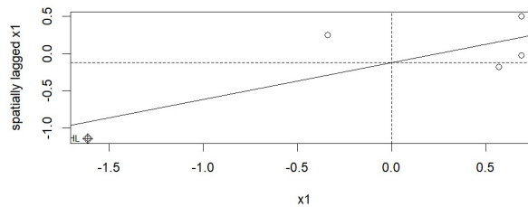
Fig. 1: Moran's I scatterplot.
