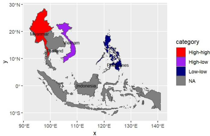
Fig. 2: LISA-based spatial clustering.
